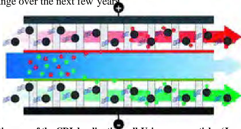
Figure 22: Diagram of the CDI desalination cell Using nanoparticles (Jeon et al. 2013).
