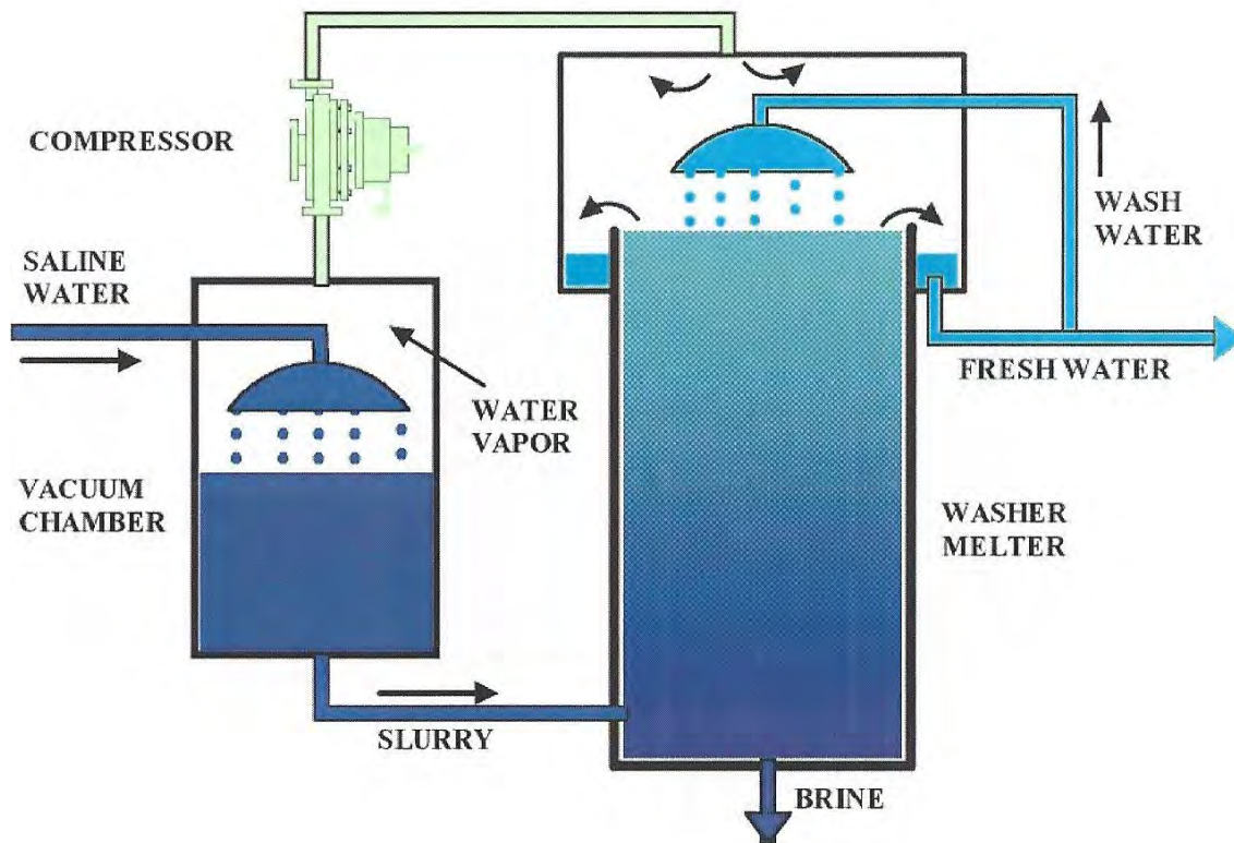
Figure 14: Vacuum freeze desalination.
